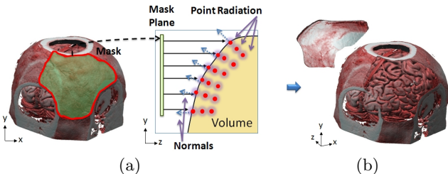
Fig. 5 (a) Peeling the skull with a free-form mask, parallel raycasting into the volume to find separate surface position and normal, and executing point radiation along the detected inverse normal directions. (b) Removing surface layers and pasting back the skull with a second rendering pass.
