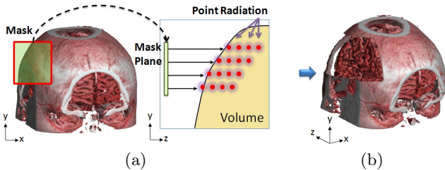
Fig. 3 (a) Drilling the super-brain data with a square mask, raycasting into the volume to find surface points, and executing point radiation along the view-direction. (b) Applying multiple pressures to cut through the skull.
