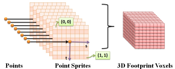
Fig. 2 Points are emitted as 2D point sprites by a single geometry program and reconstructed into 3D footprint voxels. Each 2D point sprite contains automatically generated texture coordinates ranging from (0, 0) to (1, 1) .
