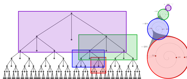
Figure 10. A tree with 190 nodes and 7 levels in both node-link and PaisleyTree layout. In PaisleyTrees, each node circle shows three levels: a node and all of its children and grandchildren.
