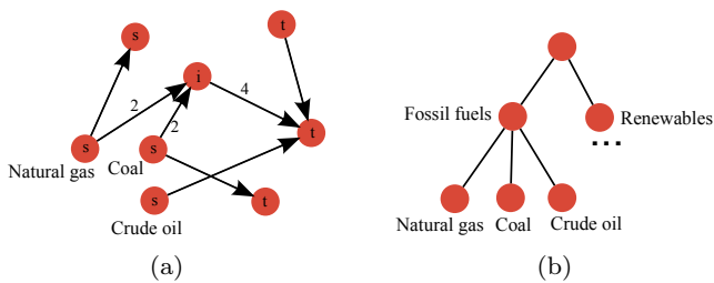
Fig. 2: (a) A sample network flow for an energy system. Source, intermediate and sink nodes are marked with s, i and t respectively. Numbers represent edge weights. (b) A sample hierarchy for an energy system network flow.
