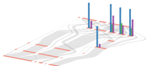
Fig. 8: Three categories of emissions shown for each node of the Sankey diagram in 3D. Blue, green and purple represent CO_2 , N_2O and CH_4 respectively.
