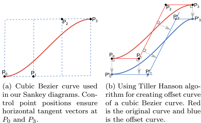
Fig. 5: Creating flows in the Sankey diagrams.
