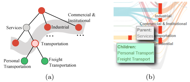
Fig. 7: Hierarchical exploration of Sankey diagram. (a) A sample hierarchy tree of data. The enclosed nodes are the current nodes visualized in the Sankey diagram. (b) The hovering interaction for hierarchy in (a). Hovering over Transportation node shows Services as parent and Personal Transportation and Freight Transportation as children.
