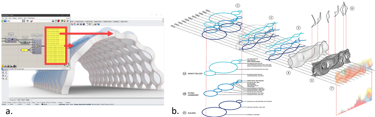
Figure 8: (a) An example of a parametric design generated by Grasshopper. The visual programming interface of Grasshopper, as well as its data list, is shown on the left. Image taken from [Son21], (b) A diagram showing parametric design stages of generating form from the original data, using Grasshopper. Image taken from [Mar14]
